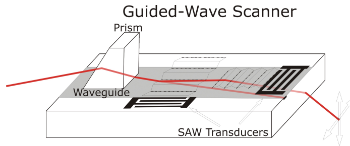
Figure 5-1: 2D Scanner
