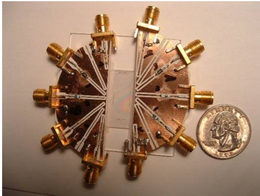
Figure 5-11: Packaged Device
