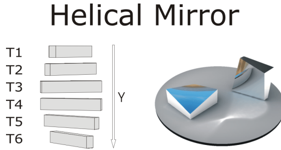
Figure A-2: A helical mirror can be thought of as a stack of long mirrors, each rotated at a slightly greater angle. Each of these mirrors represents a scanning mirror frozen at a different time, so that moving a beam vertically up and down the mirror is, in an HPO (Horizontal Parallax Only) system, the same as reflecting a beam of a single mirror that is rotating (rendering by Quinn Smithwick).
