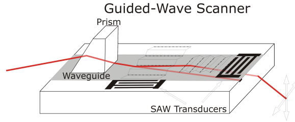
Figure 2-8: The Guided Wave Scanner
