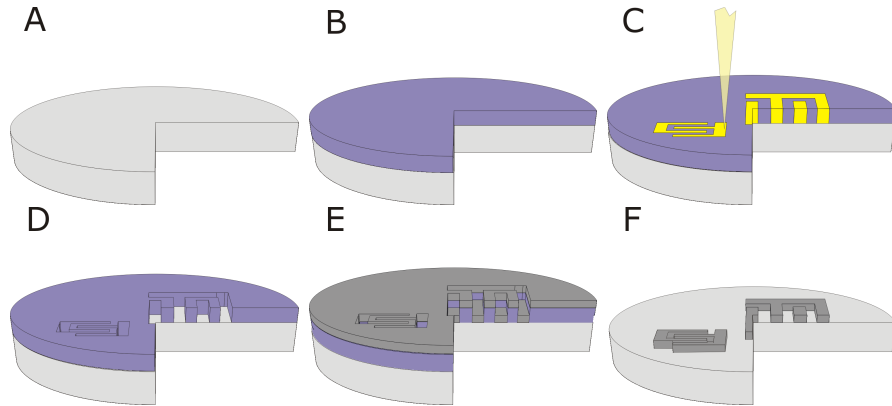
Figure 5-3: Mask Making Steps (A) Start with a blank fused-silica wafer (B) Spin 300nm PMMA (C) Ebeam write the transducer pattern (D) Develop exposed pattern in IPA:MIBK (E) Deposit Chromium (F) Lift-off PMMA in Acetone
