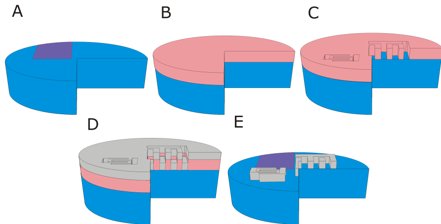
Figure 5-7: Transducer Fabrication Steps (A) Start with Proton Exchanged Lithium Niobate (B) Spin Negative Resist (C) Use flex mask to pattern resist (D) Deposit Aluminum (E) Liftoff resist with Acetone
