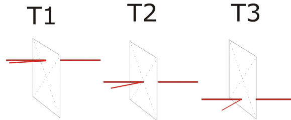
Figure A-3: Function of the HOE—light will diffract at a larger angle when passing through the bottom of the HOE than the top.
