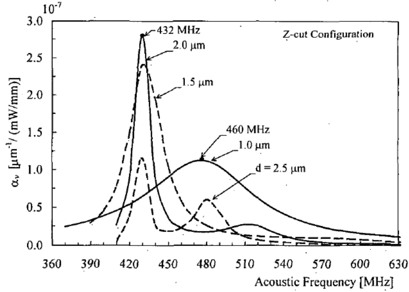
Figure 4-5: Mode coupling spectrum for different waveguide depths (from Matteo[1])
