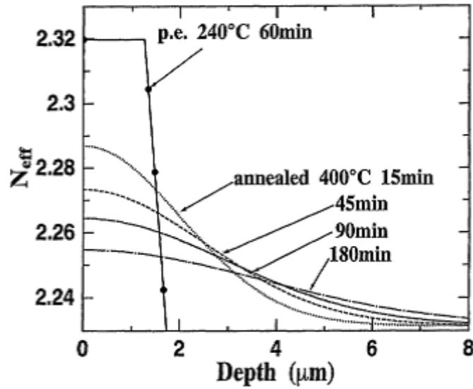
Figure 4-4: Alteration waveguide profile with anneal time (from Kakio[2])
