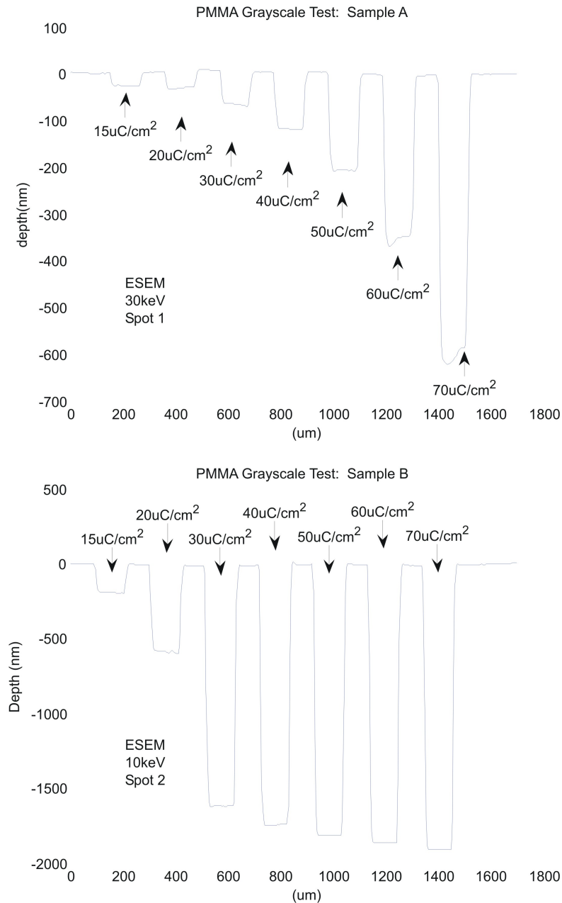
Figure A-7: Both samples above where written with the same ebeam dose the differing depths result from the fact that more energy was imparted to the film in the 10keV case.
