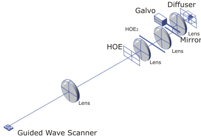
Simplified drawing of the Mark III holographic video display
