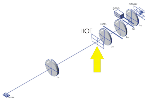
Mark III Hologvideo System
