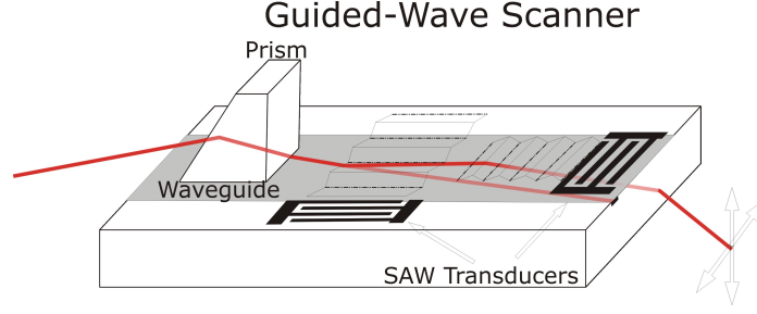
Figure 1-2: 2D Scanner
