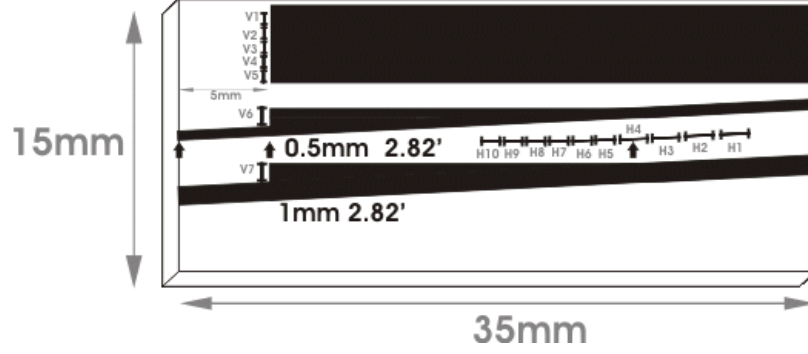
Figure 4-11: Waveguide and transducer layout. Notice that there are extra transducers and waveguides above and below the central waveguide that serve as test structures.
