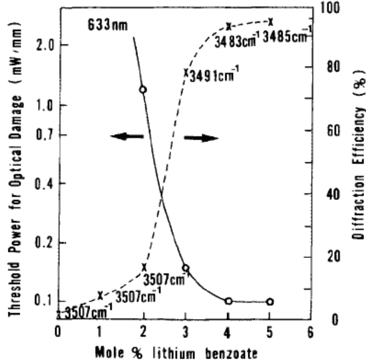
Figure 4-2: Optical damage threshold with melt dilution (from Miyawaki[3])
