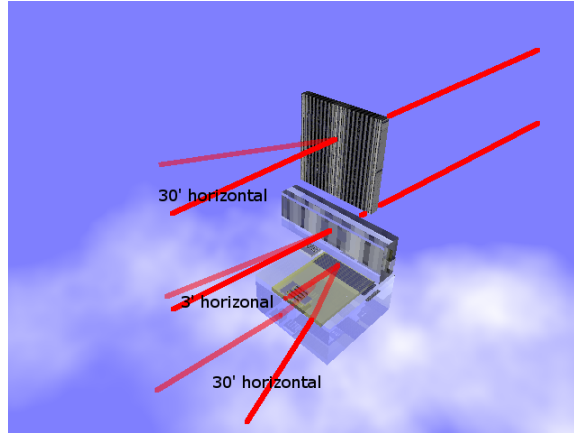
Figure 2-7: The hologram (top) has high spatial resolution and can therefore diffract over large angles. The AOM (middle) and other modulators like DMDs and LCDs have a spatial resolution that is approximately ten times smaller than a typical hologram and their ability to diffract is proportionally lower. One of the goals of my work with the Guided Wave Scanner (bottom) is to create a modulator with a spatial frequency on the order of a typical hologram, capable of equivalently large angles of diffraction.
