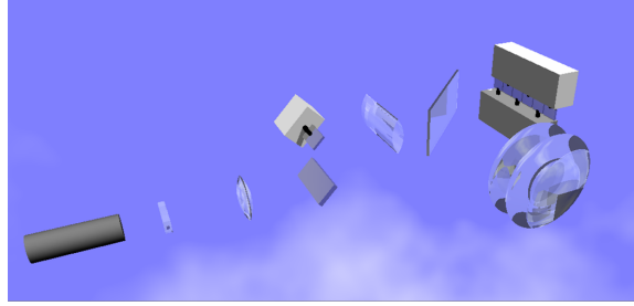
Figure 2-2: The Mark II optical geometry
