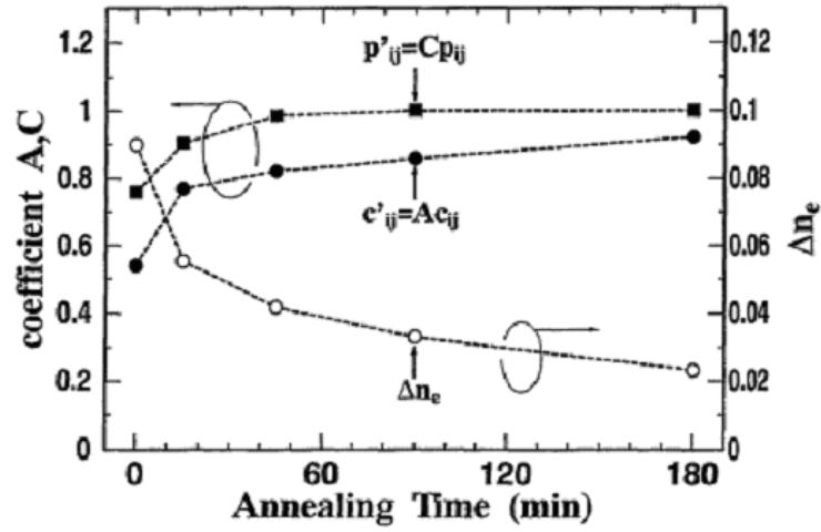
Fig. 6. p'_{ij} , c'_{ij} and \Delta n_e dependence on annealing time.
