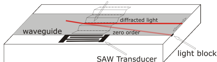
Figure 1-4: Non-collinear, in-guide diffraction
