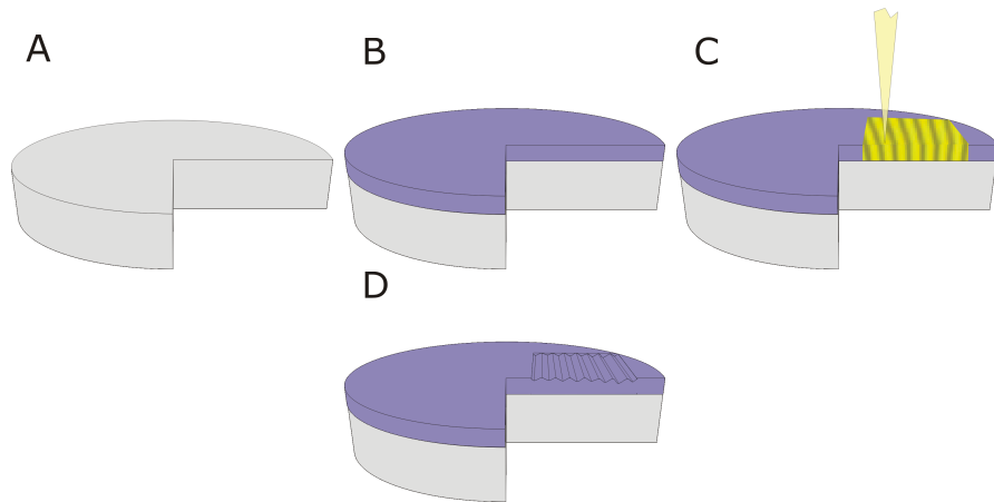
Figure A-5: HOE Fabrication Steps (A) Start with a blank fused-silica wafer (B) Spin 300nm PMMA (C) Ebeam write (with varying dose) the HOE pattern (D) Develop exposed pattern in IPA:MIBK
