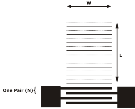
Figure 4-7: Transducer parameters
