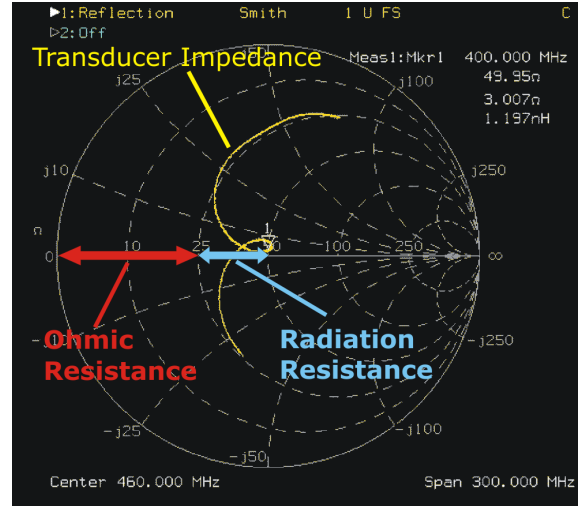
Figure 5-10: This figure shows the network analyzer’s Smith chart output for the second horizontal transducer, H2. The transducer’s impedance is shown looping near 50\Omega . The ohmic resistance corresponds to the ohmic loss of the device. The radiation resistance corresponds to the proportion of the electrical power that is converted to acoustic waves and radiated away from the transducer. Notice that the radiation resistance is greatest near the center frequency of the transducer.
