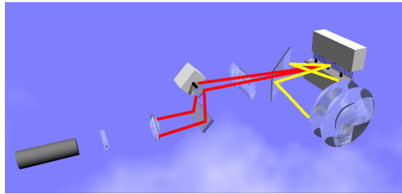
Figure 2-3: Highlighted, is the telescope system responsible for demagnification in the Mark II geometry
