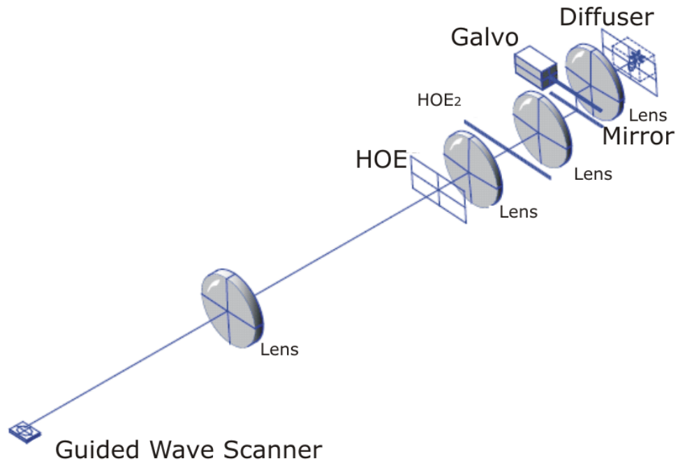
Figure 2-9: The Mark III Holovideo Geometry (Courtesy of Quinn Smithwick)
